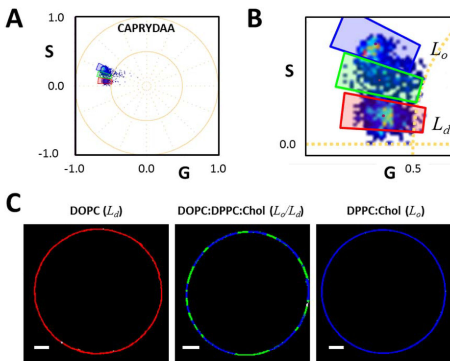
Figure 7: CAPRYDAA fluorescence in GUVs with different phases.
