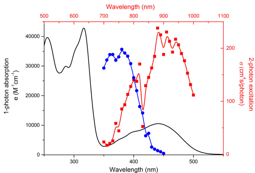
Figure 4. Two-photon excitation spectra for CAPRYDAA and LAURDAN:
