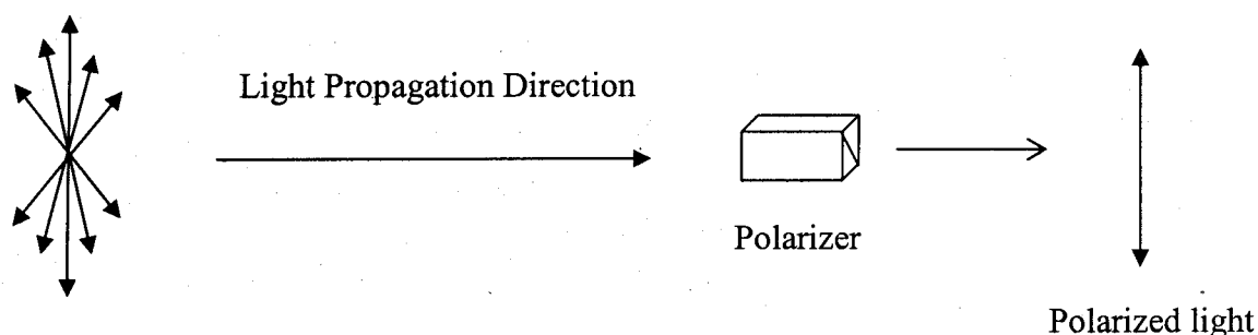
Fig. (1). Diagram showing the orientation of electric vectors in natural light and the isolation of vertical polarized light through a polarizer.
