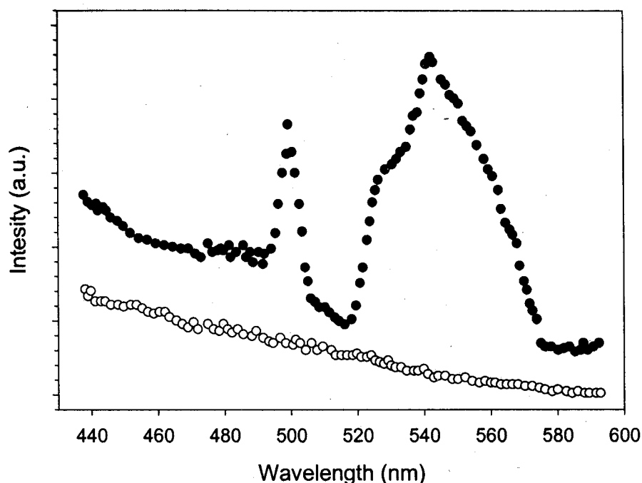
Fig. (5). Demonstration of parasitic light (Rayleigh Ghosts) in a meter Jarrell-Ash monochromator (data was obtained on the photon-counting instrument described in [9]). Upper trace (closed circles) - buffer solution, excited at 350nm and scanned from 436-595nm. Lower trace (open circles) - the same scan but with a cut-on filter, which blocked wavelengths below 400nm, placed between the sample and the emission monochromator to prevent the 350nm scatter from entering the monochromator.
