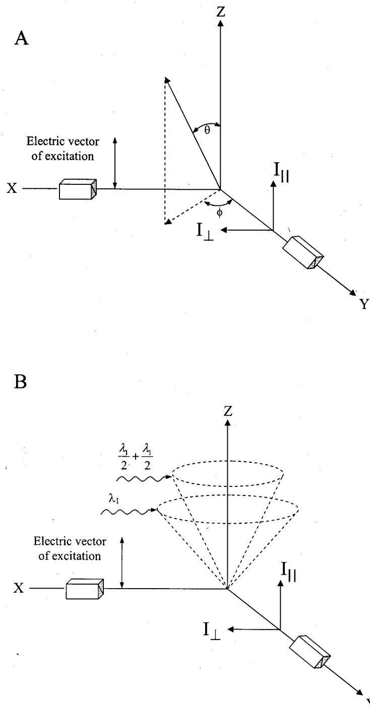
Fig. (2). A. Diagram depicting (a) photoselection of an absorption dipole, making angles \theta with the Z-axis (in the XZ plane) and \phi with the Y-axis (in the XY plane) by vertically polarized light and (b) observation along the Y-axis of the vertical (parallel) and horizontal (perpendicular) components of the emission through a polarizer. B. Depiction of the photoselection process for one- and two-photon excitation.
